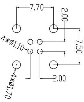
PCB Layout Reference
